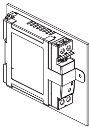
Mounting facing horizontally with S82Y-VS30P*
