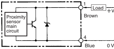
E2E-X□D1 Without Diagnostic Output
