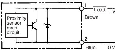
E2E-X□D2 Without Diagnostic Output
